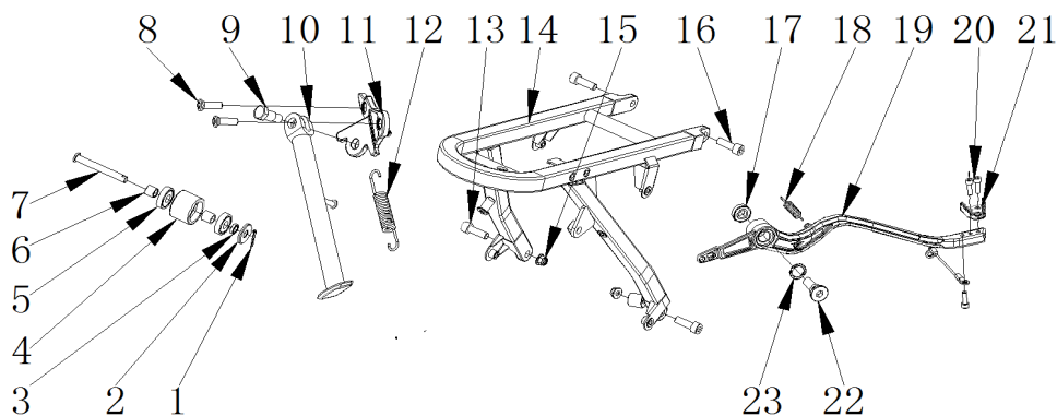
踏脚/脚撑 FOOT PEGS / SIDE STAND
