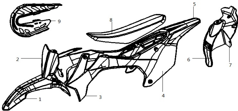
车体盖 SEAT / PLASTICS
