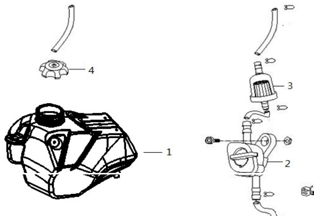
油箱/油开关 FUEL TANK/FUEL COCK
